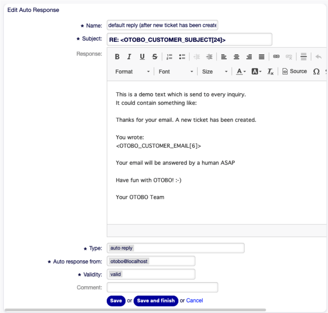
Fig. 1.8: Edit Auto Response Screen
