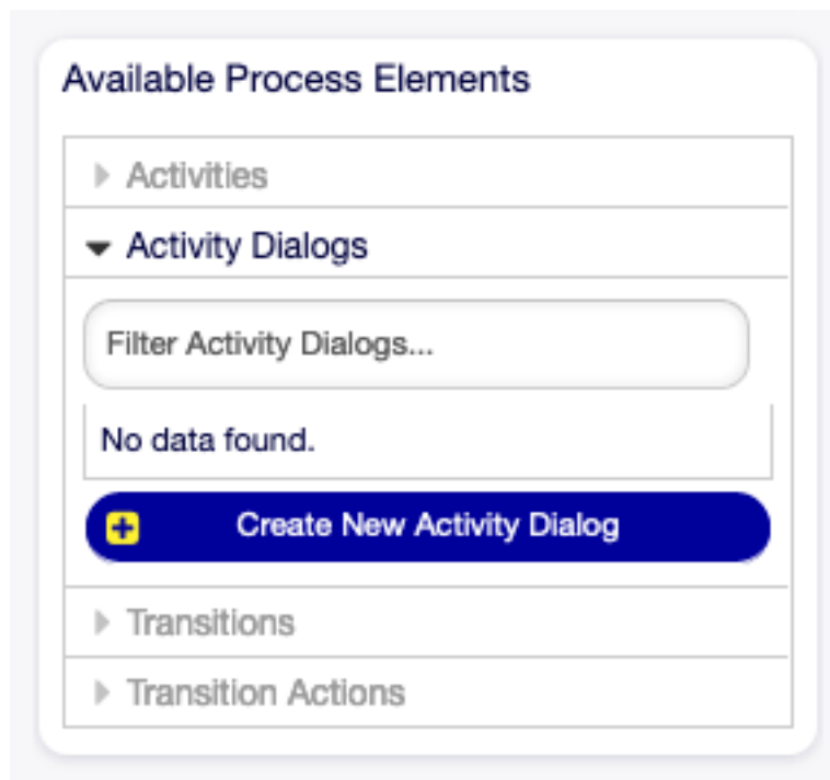
Fig. 1.199: Book Ordering - Activity Dialogs
